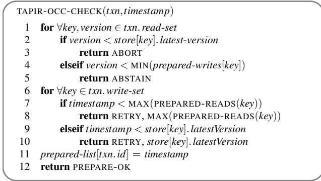
Figure 8: Validation function for checking for OCC conflicts on Prepare . PREPARED-READS and PREPARED-WRITES get the proposed timestamps for all transactions that the replica has prepared and read or write to key , respectively.
